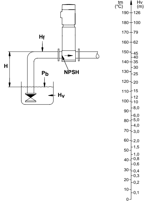
Fig. 25 Minimum inlet pressure - NPSH
